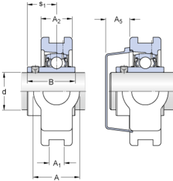
TU 1.5/16 TF Bearing 2D drawings and 3D CAD models
